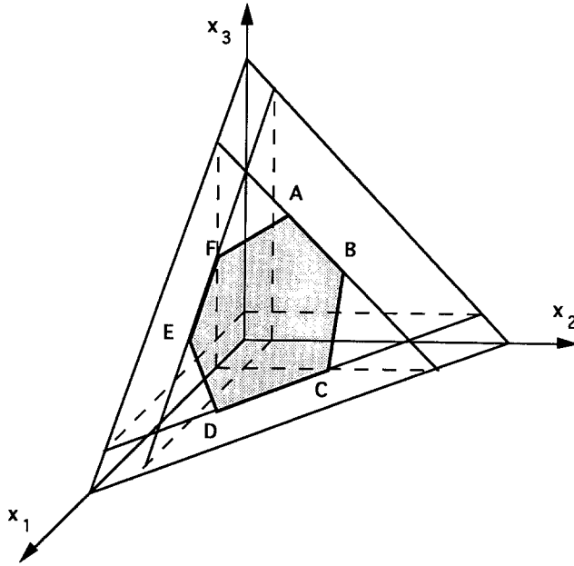
Fig. 2. An extended contra-polymatroid in dimension 3.
